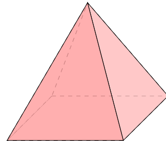
square-based pyramid
